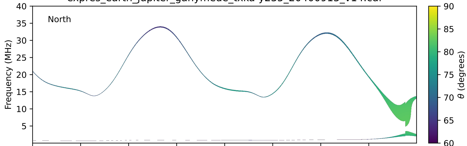
expres_earth_jupiter_ganymede_txka-y235_20400913_v14.cdf
