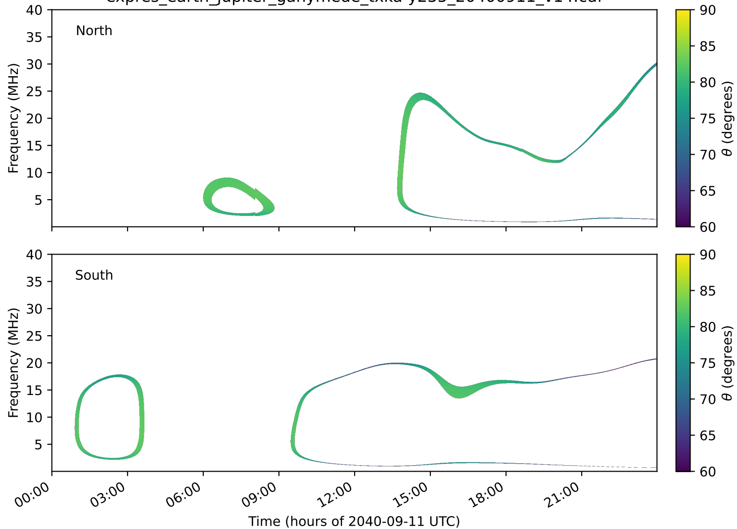
expres_earth_jupiter_ganymede_txka-y235_20400911_v14.cdf
