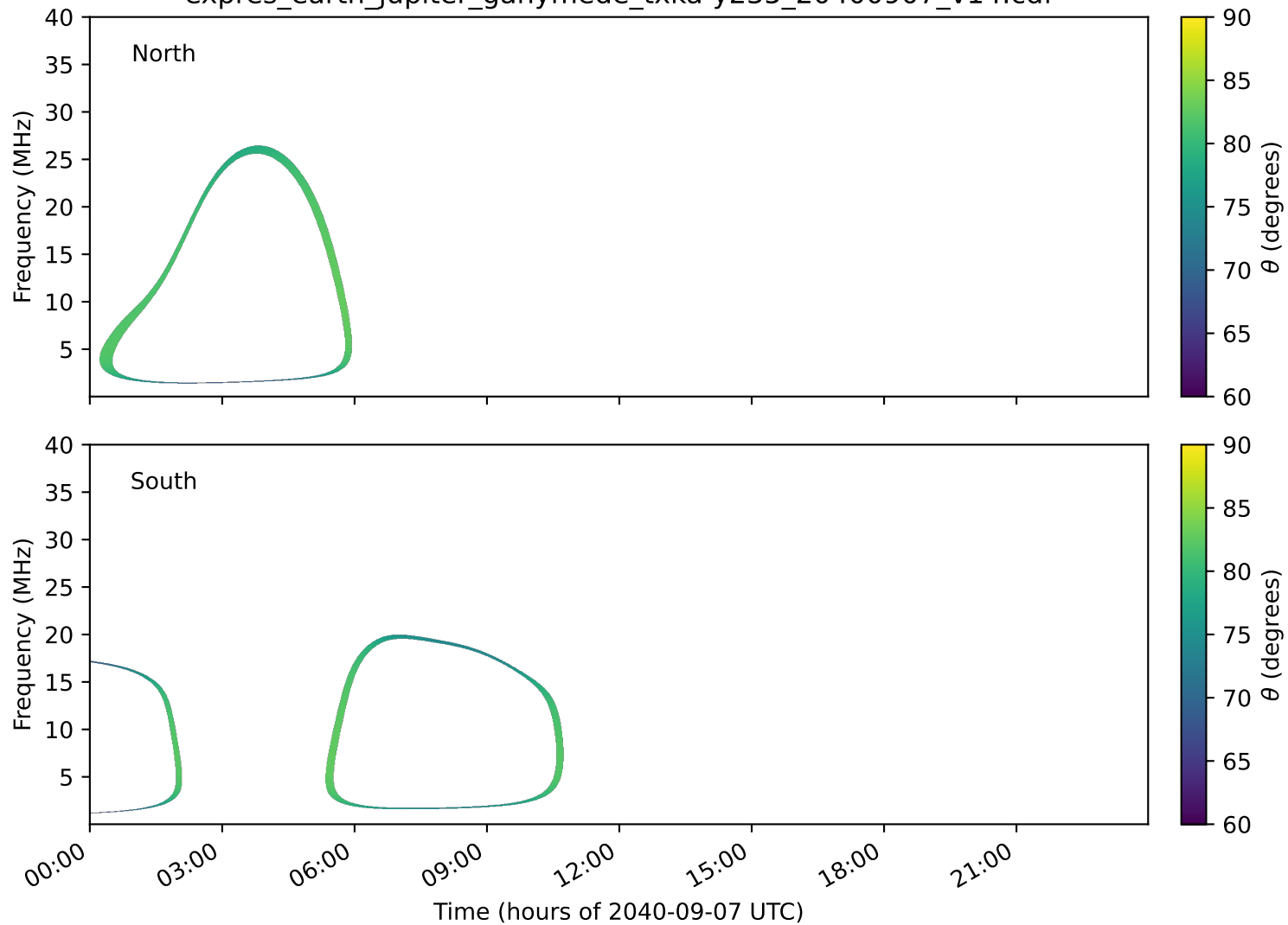
expres_earth_jupiter_ganymede_txka-y235_20400907_v14.cdf
