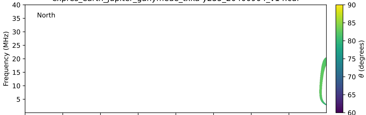
expres_earth_jupiter_ganymede_txka-y235_20400904_v14.cdf
