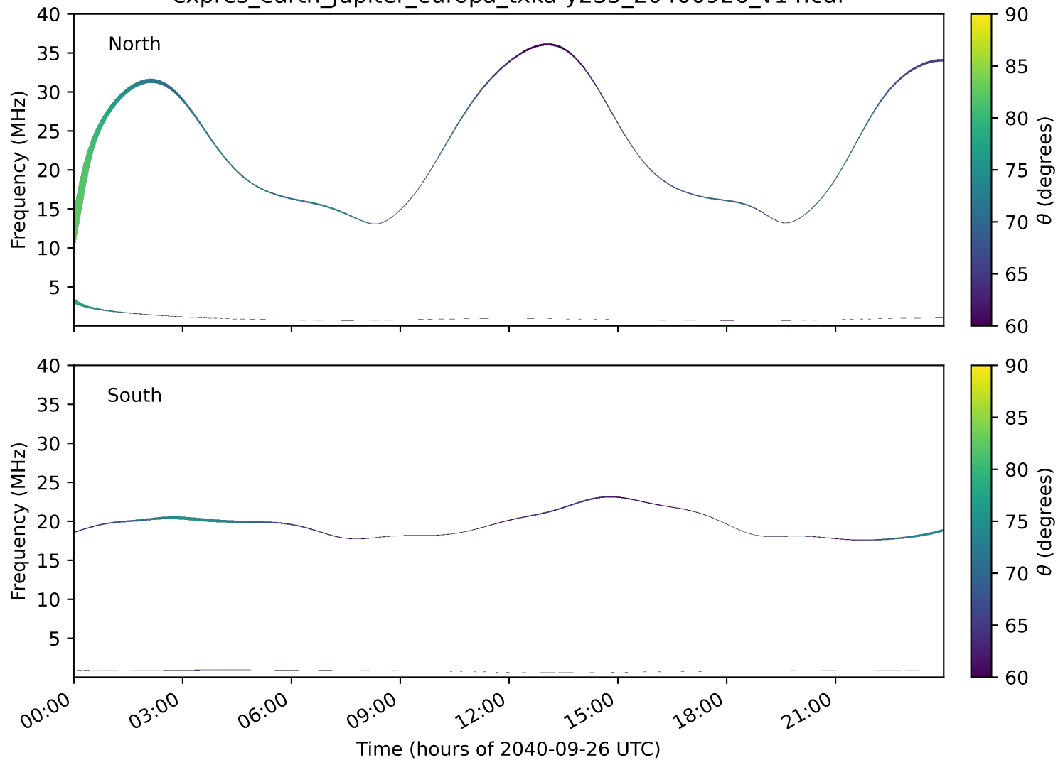
expres_earth_jupiter_europa_txka-y235_20400926_v14.cdf
