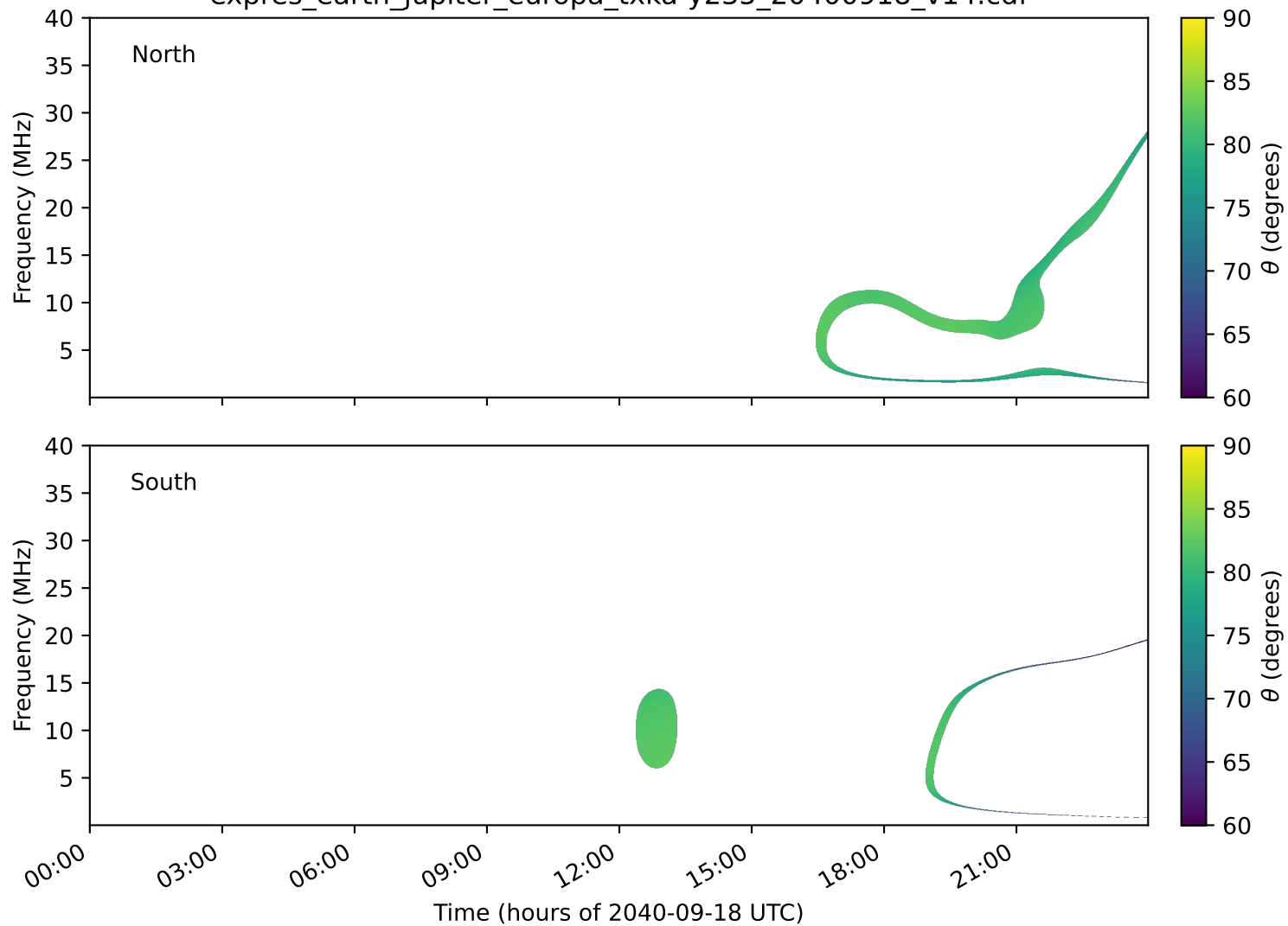
expres_earth_jupiter_europa_txka-y235_20400918_v14.cdf
