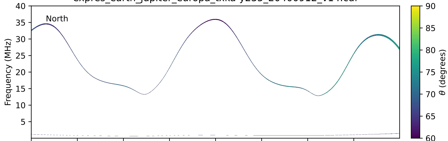
expres_earth_jupiter_europa_txka-y235_20400912_v14.cdf
