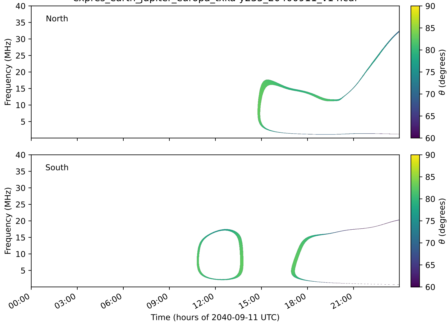
expres_earth_jupiter_europa_txka-y235_20400911_v14.cdf
