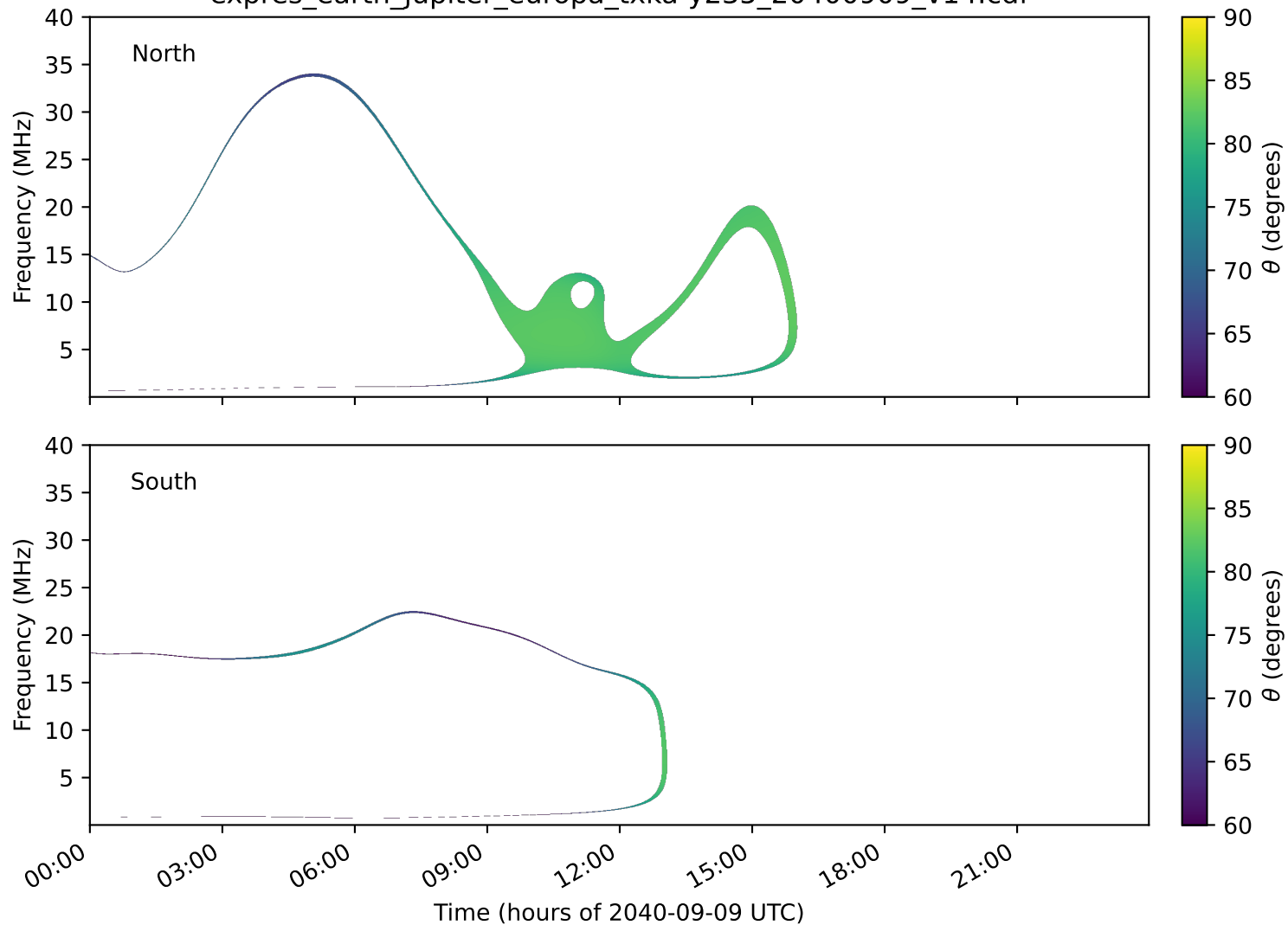
expres_earth_jupiter_europa_txka-y235_20400909_v14.cdf
