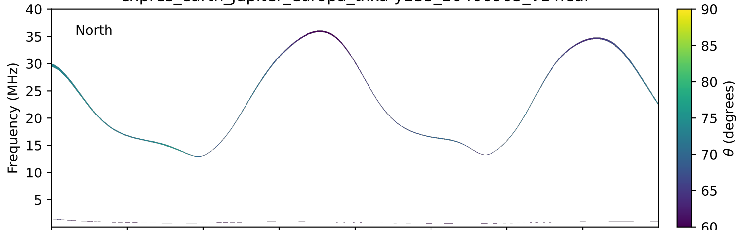
expres_earth_jupiter_europa_txka-y235_20400905_v14.cdf
