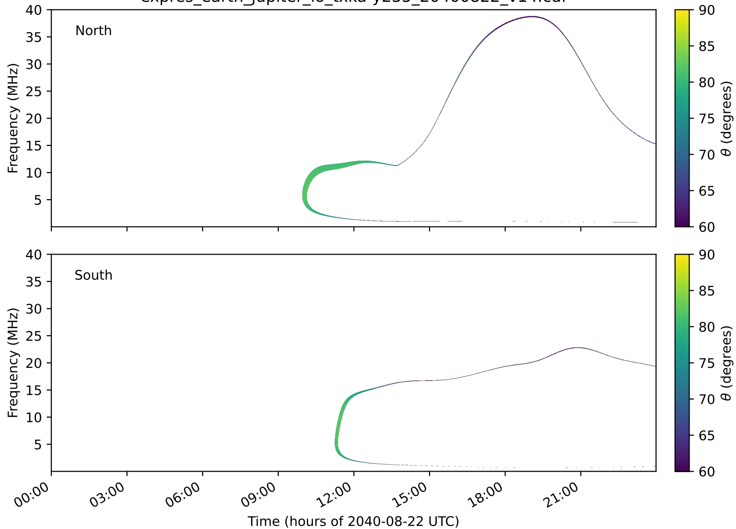
expres_earth_jupiter_io_txka-y235_20400822_v14.cdf
