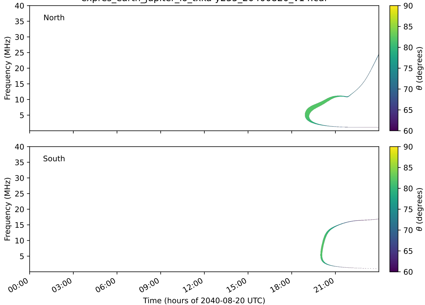
expres_earth_jupiter_io_txka-y235_20400820_v14.cdf
