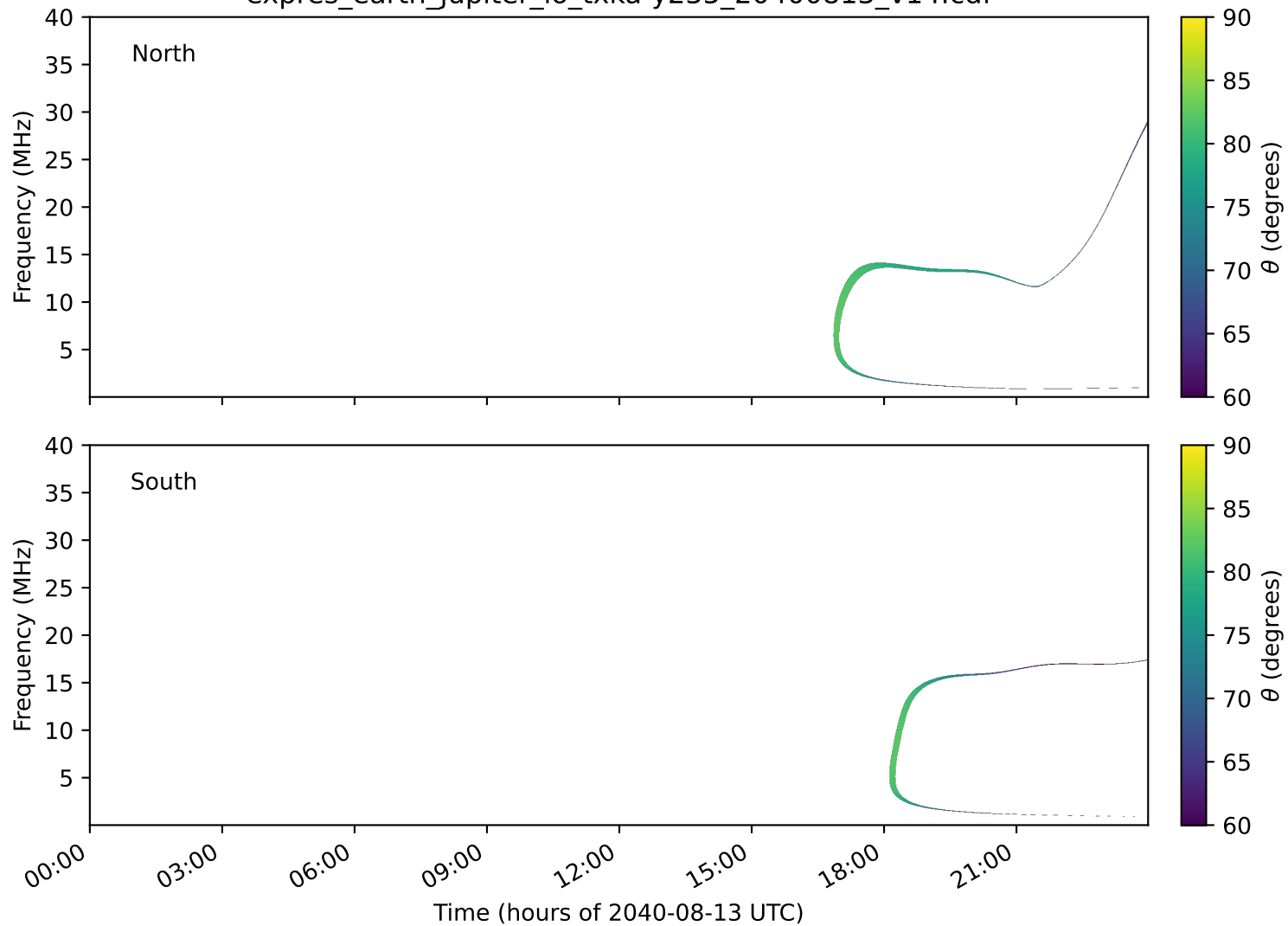
expres_earth_jupiter_io_txka-y235_20400813_v14.cdf
