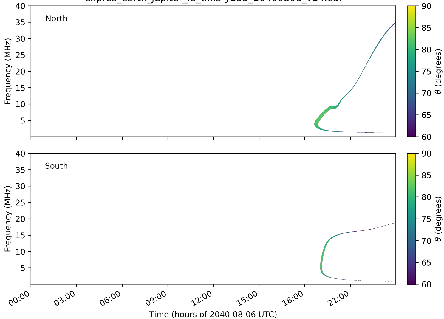
expres_earth_jupiter_io_txka-y235_20400806_v14.cdf
