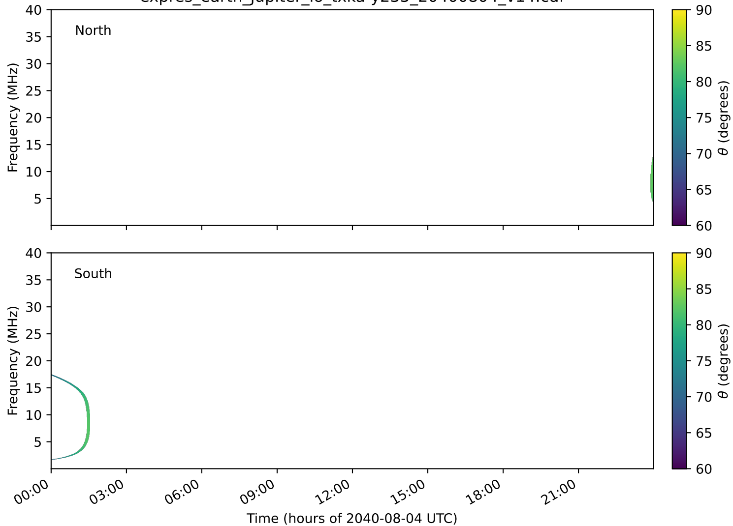
expres_earth_jupiter_io_txka-y235_20400804_v14.cdf
