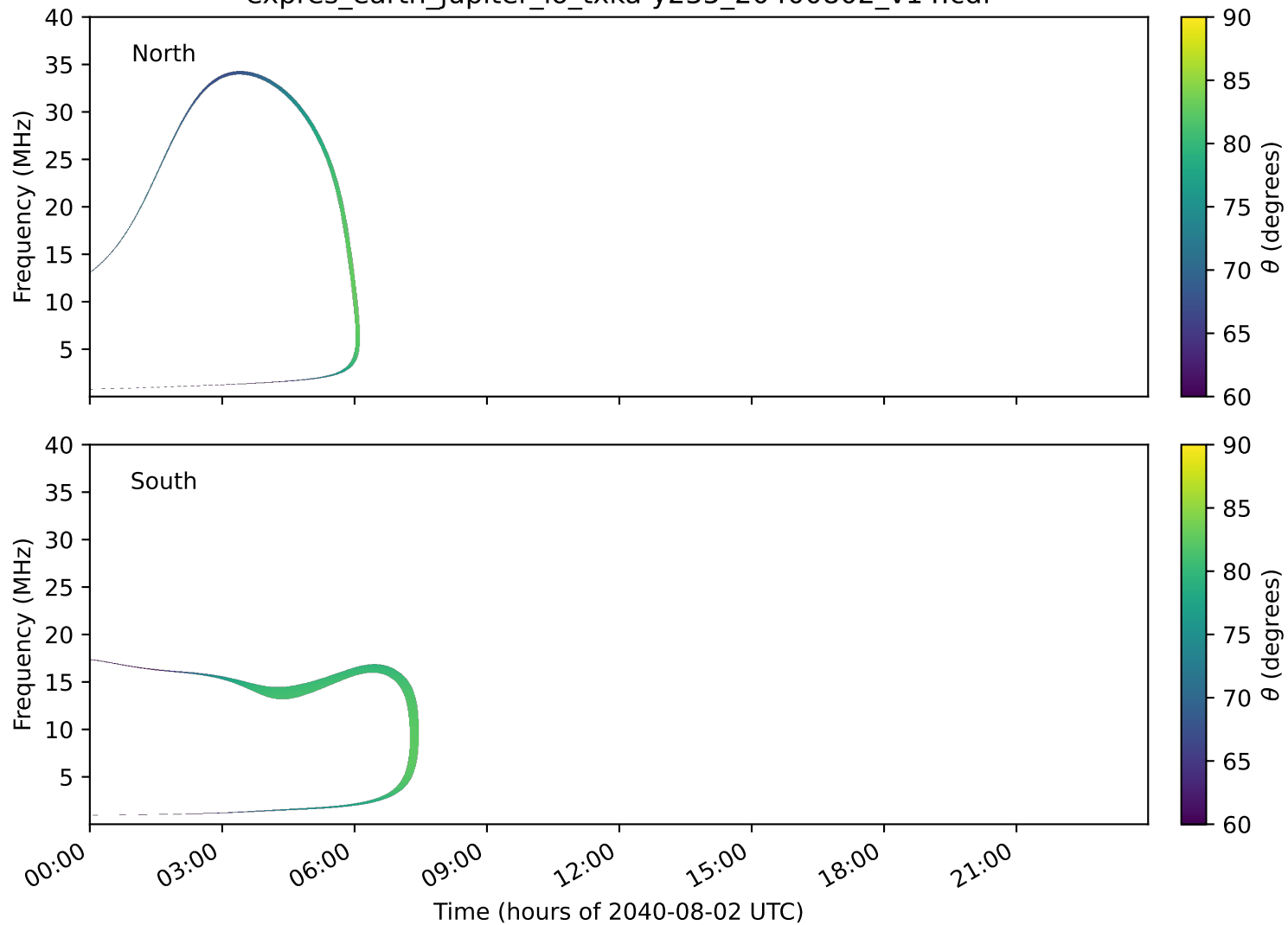
expres_earth_jupiter_io_txka-y235_20400802_v14.cdf
