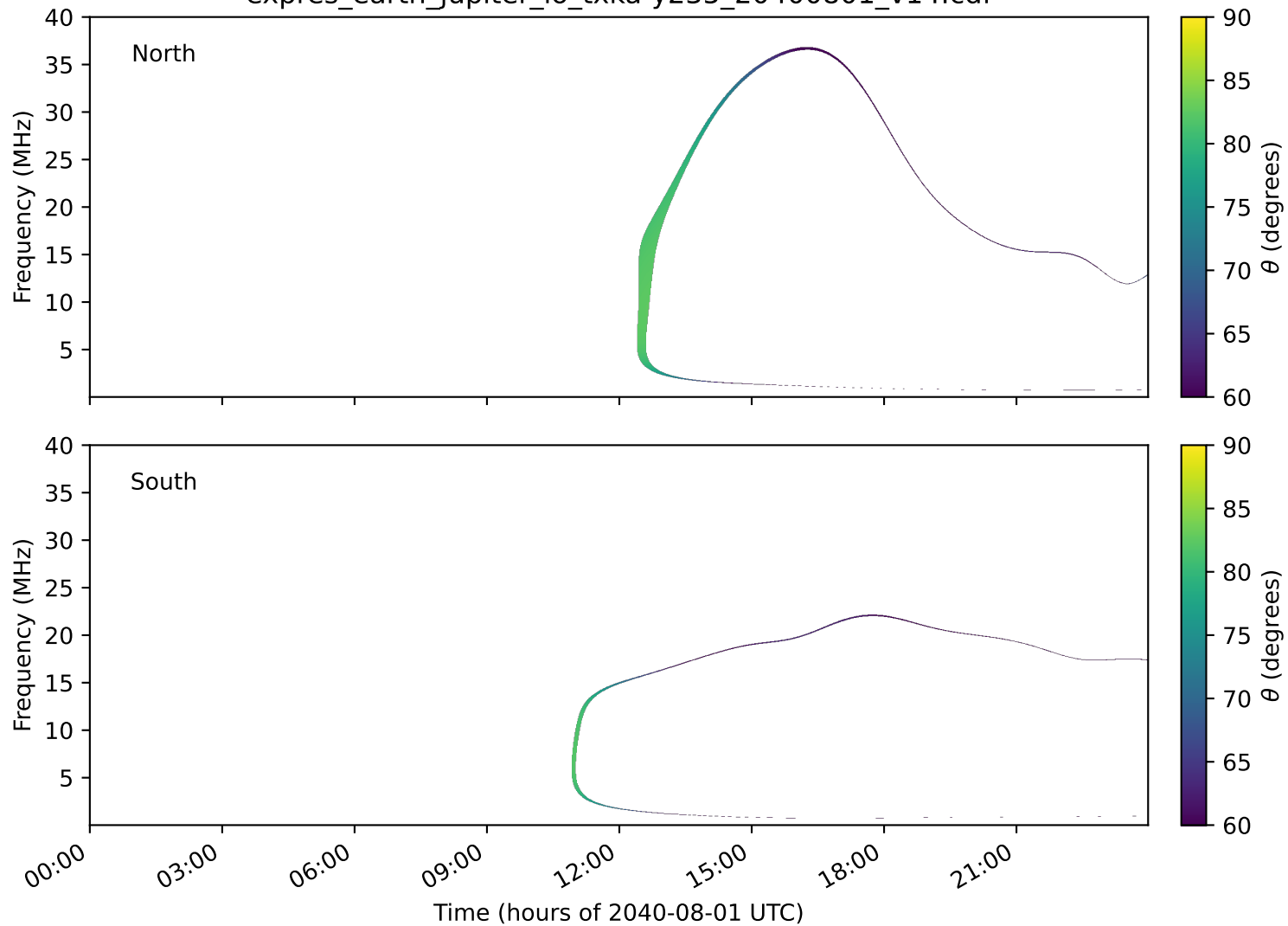
expres_earth_jupiter_io_txka-y235_20400801_v14.cdf
