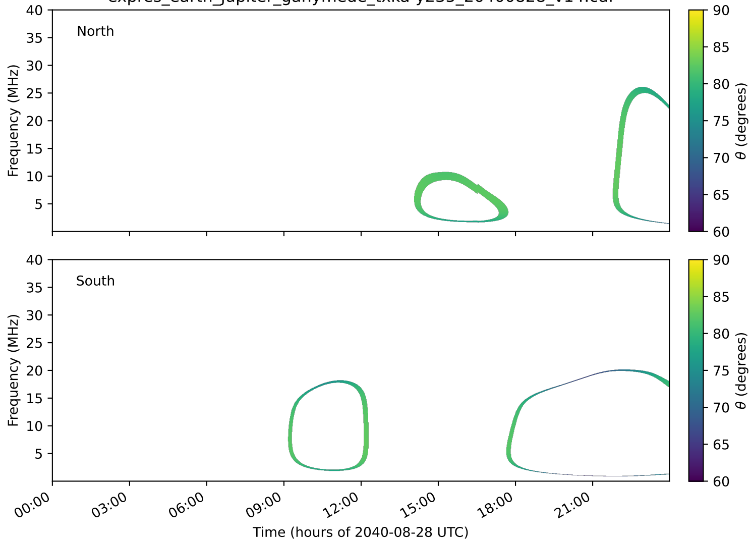
expres_earth_jupiter_ganymede_txka-y235_20400828_v14.cdf
