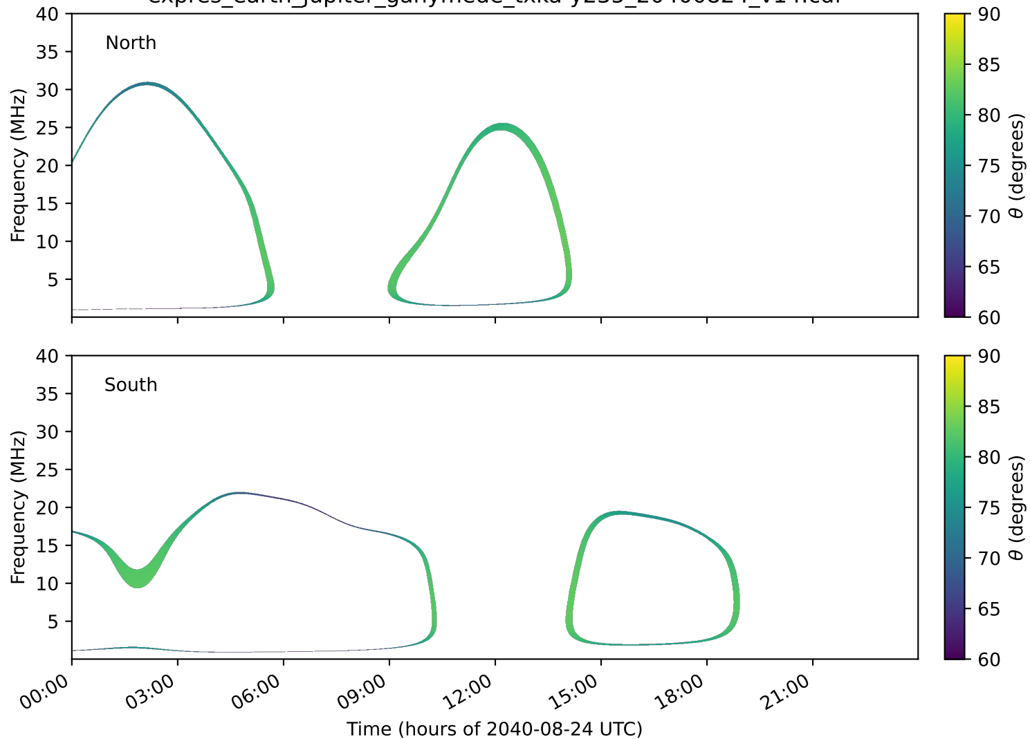
expres_earth_jupiter_ganymede_txka-y235_20400824_v14.cdf
