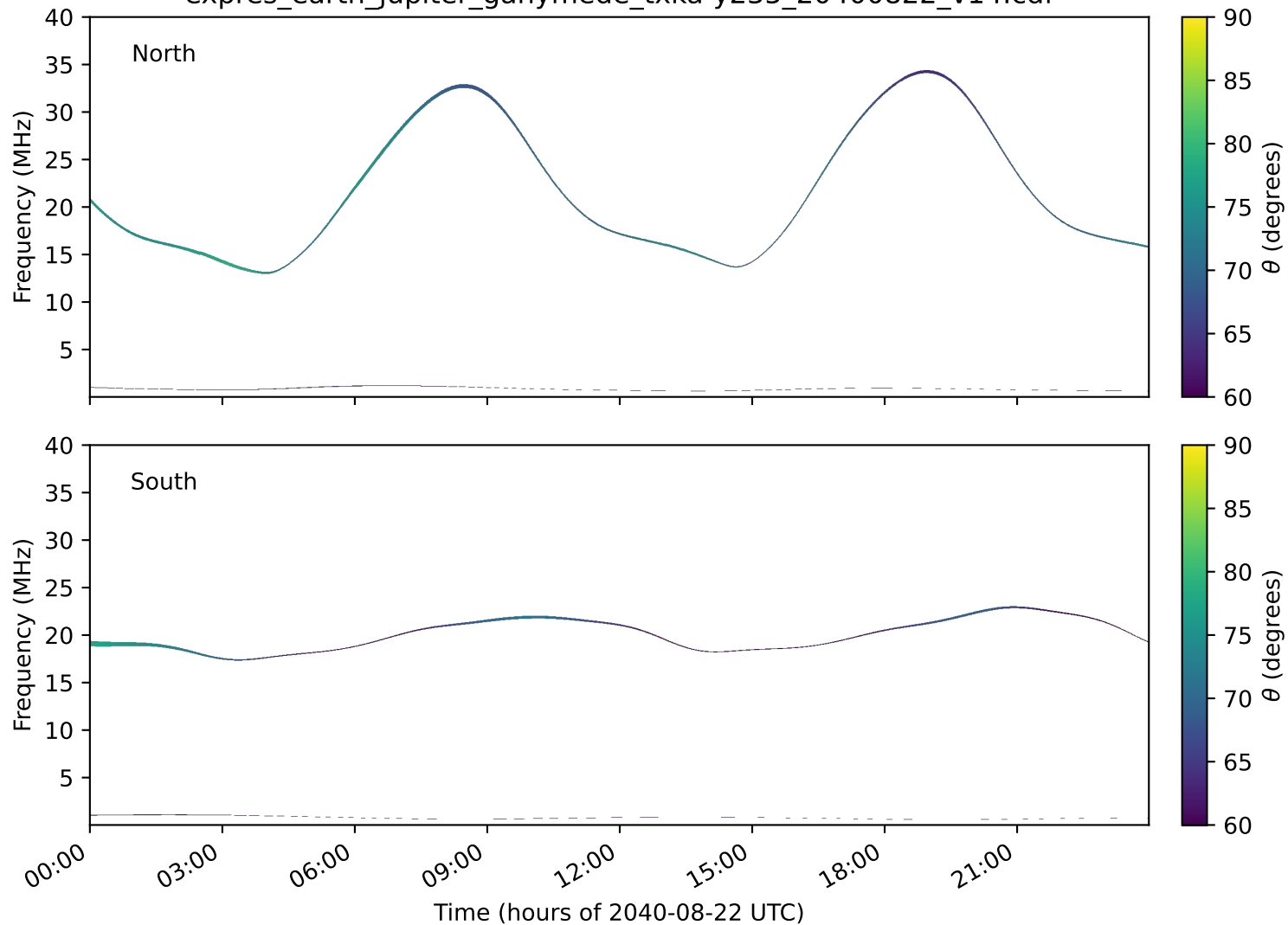
expres_earth_jupiter_ganymede_txka-y235_20400822_v14.cdf
