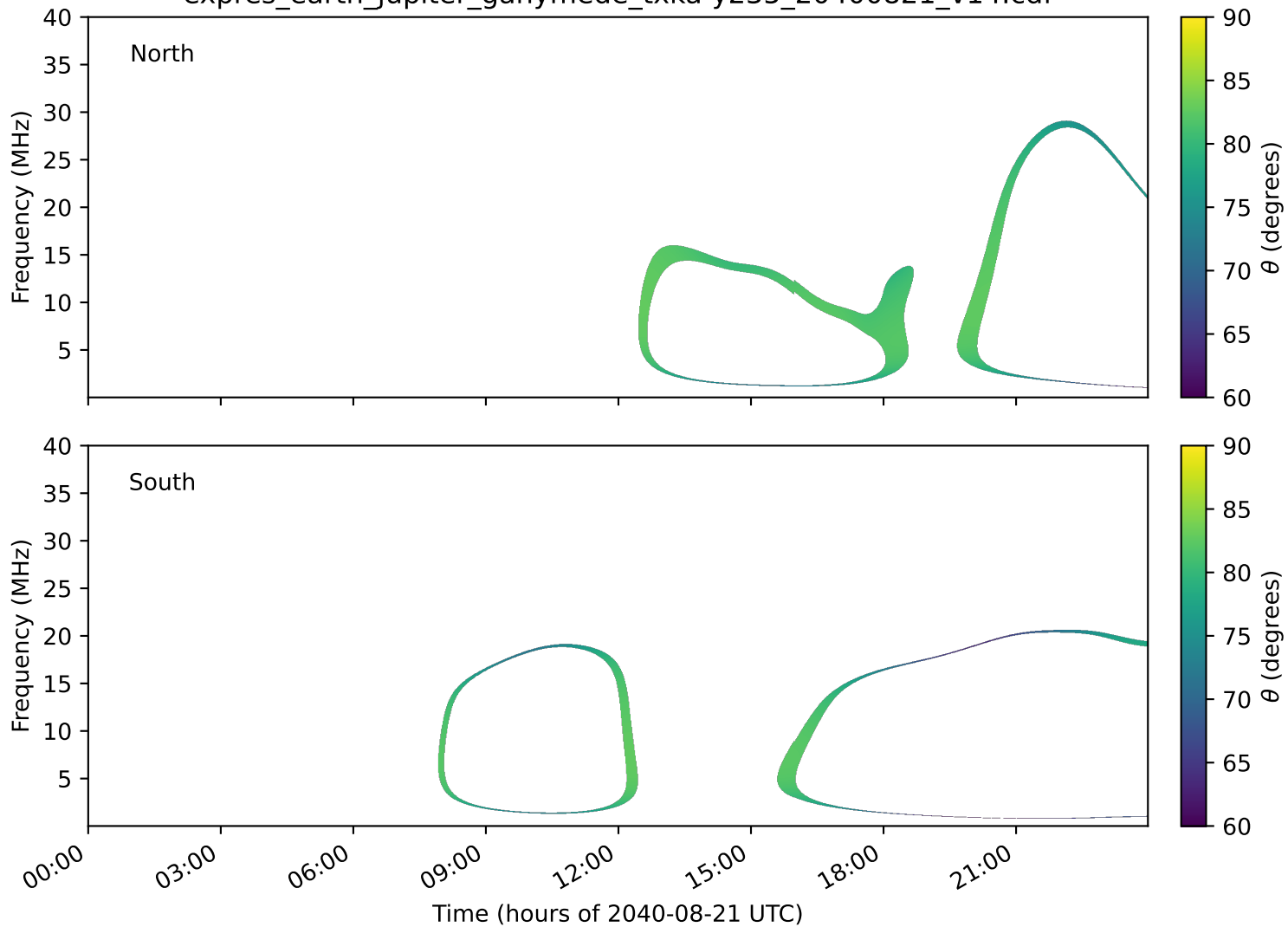
expres_earth_jupiter_ganymede_txka-y235_20400821_v14.cdf
