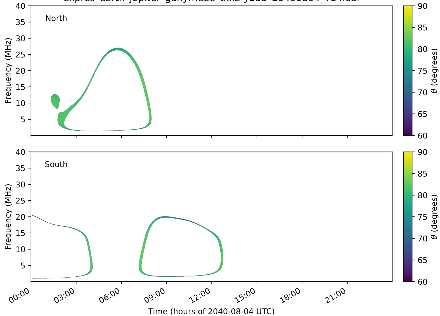
expres_earth_jupiter_ganymede_txka-y235_20400804_v14.cdf
