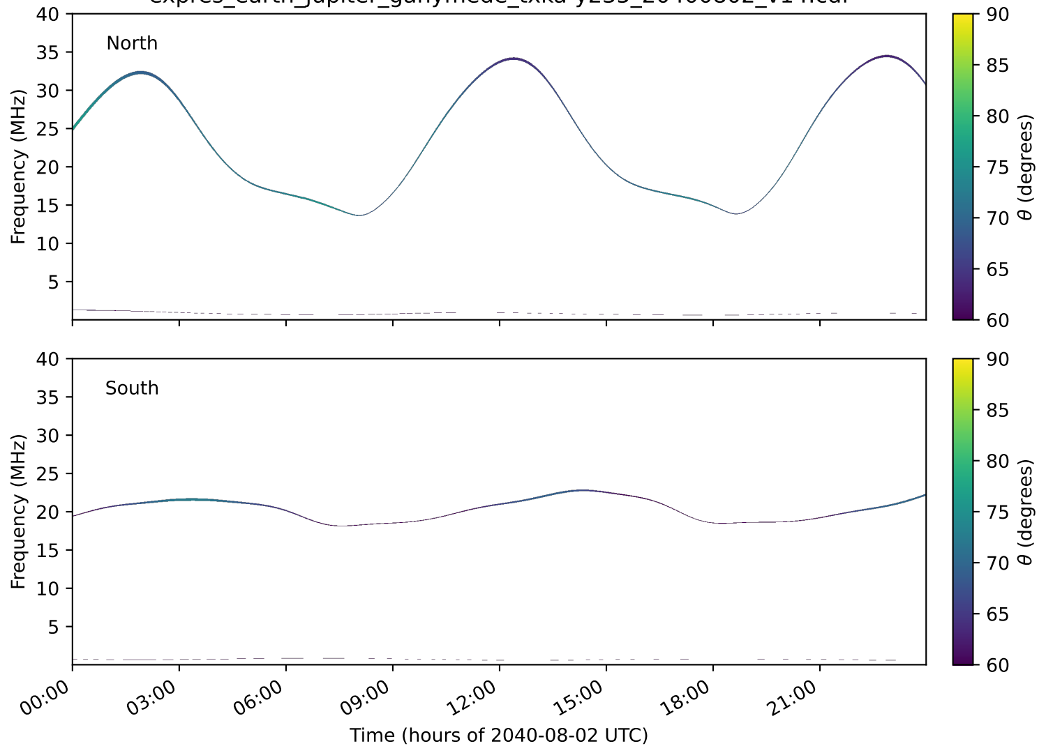
expres_earth_jupiter_ganymede_txka-y235_20400802_v14.cdf
