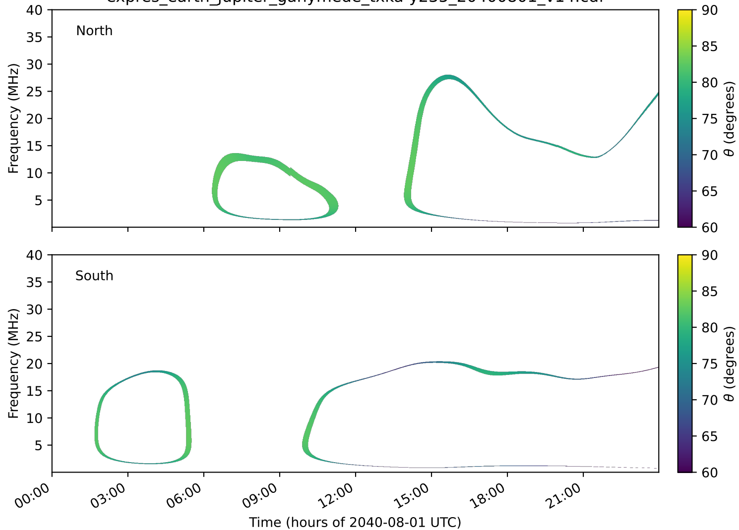
expres_earth_jupiter_ganymede_txka-y235_20400801_v14.cdf
