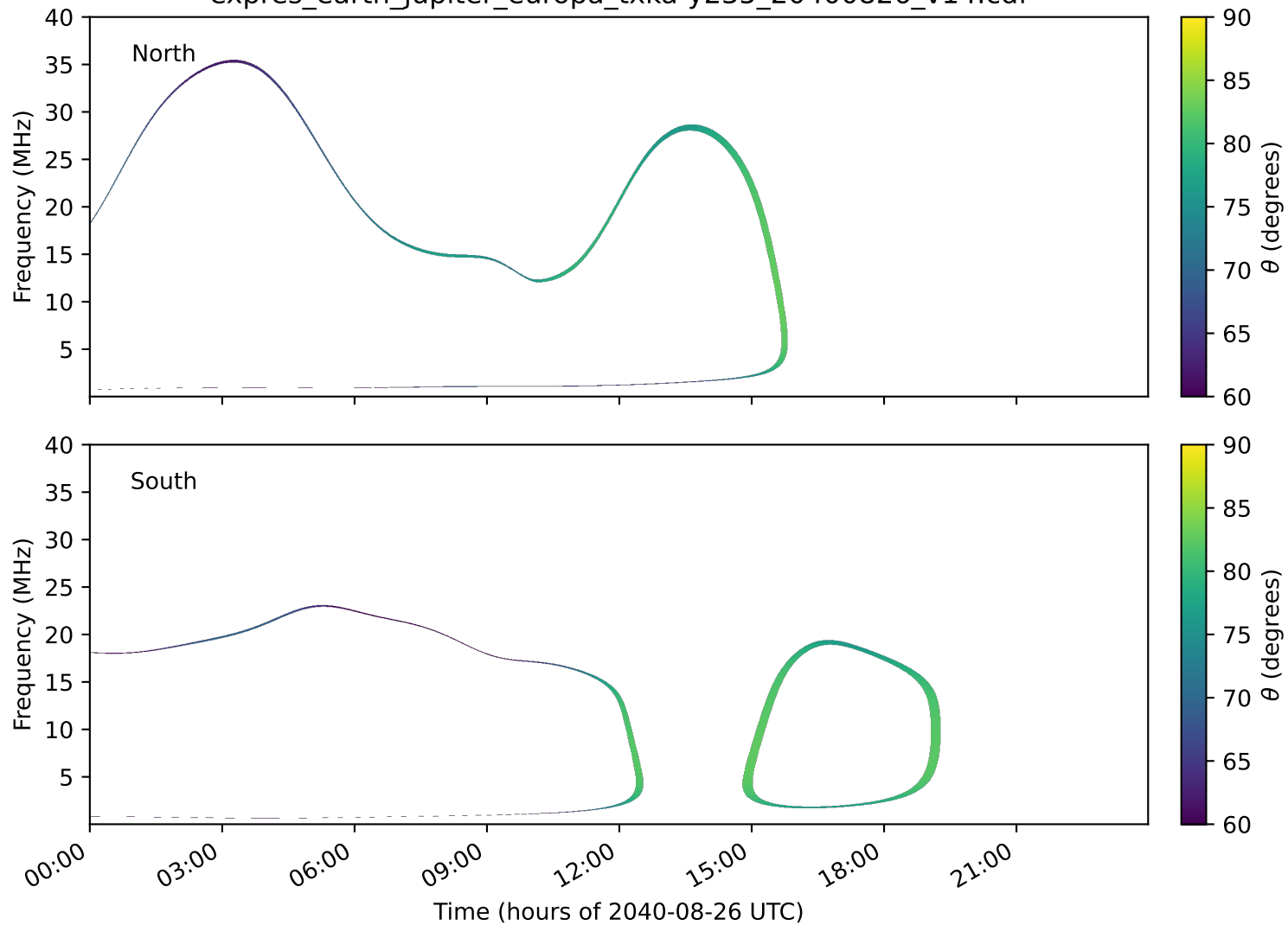
expres_earth_jupiter_europa_txka-y235_20400826_v14.cdf
