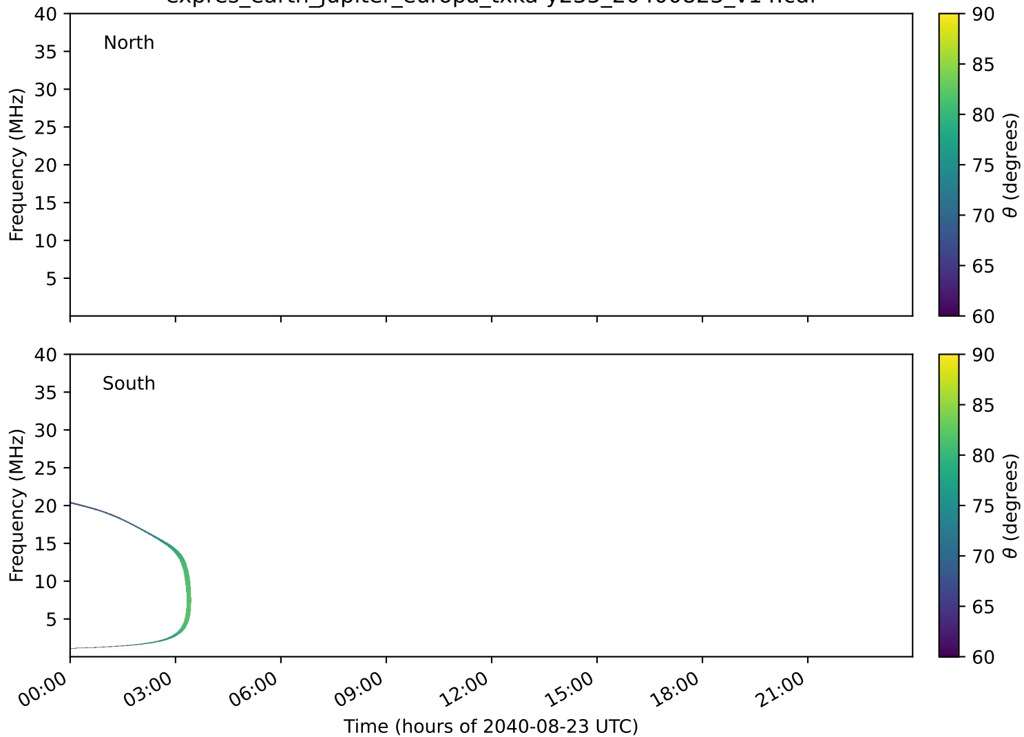
expres_earth_jupiter_europa_txka-y235_20400823_v14.cdf
