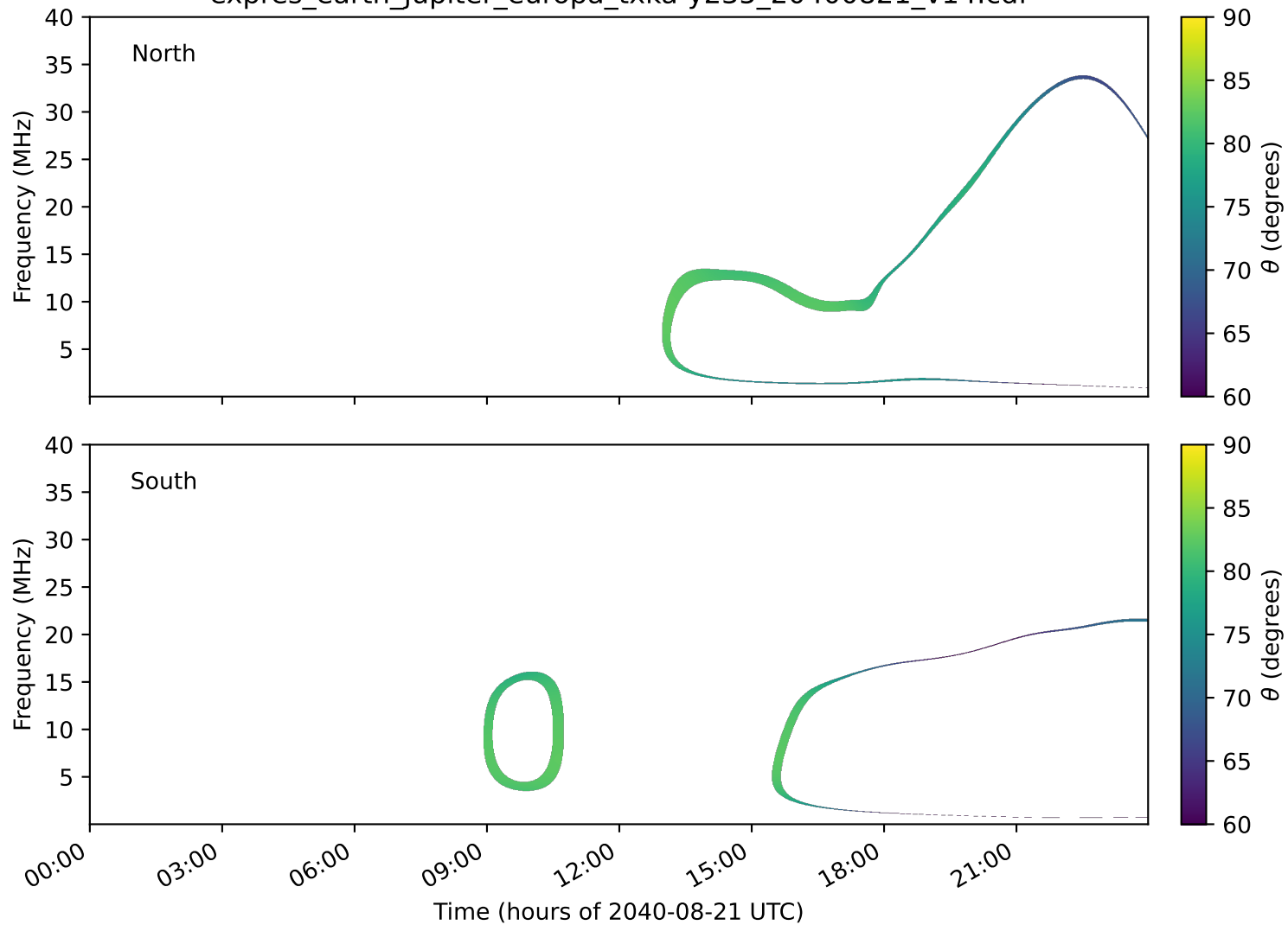
expres_earth_jupiter_europa_txka-y235_20400821_v14.cdf
