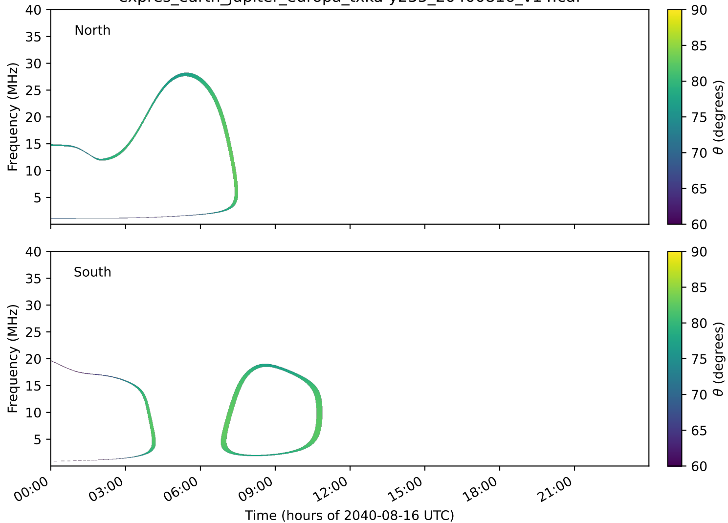
expres_earth_jupiter_europa_txka-y235_20400816_v14.cdf
