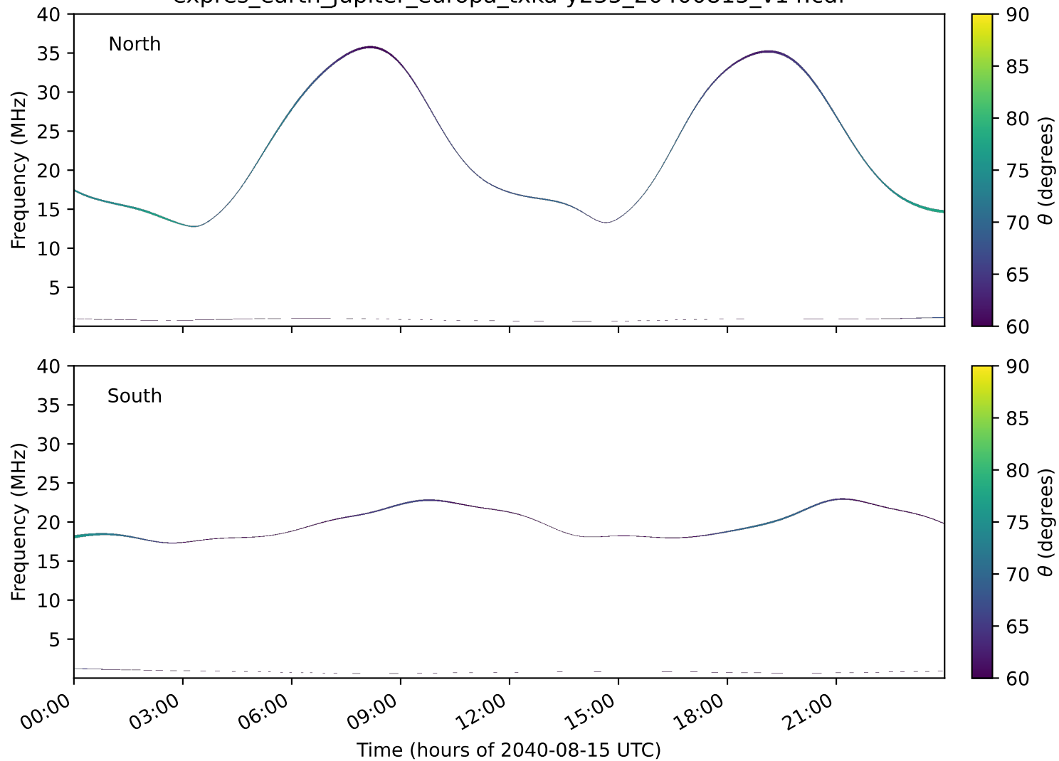
expres_earth_jupiter_europa_txka-y235_20400815_v14.cdf
