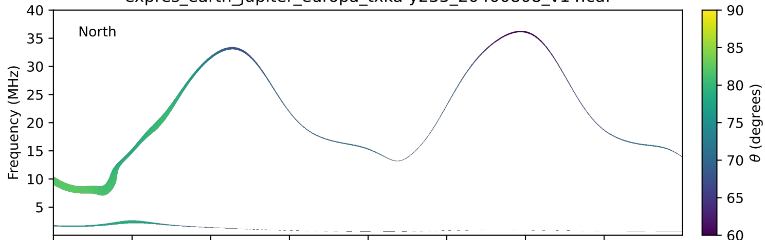
expres_earth_jupiter_europa_txka-y235_20400808_v14.cdf
