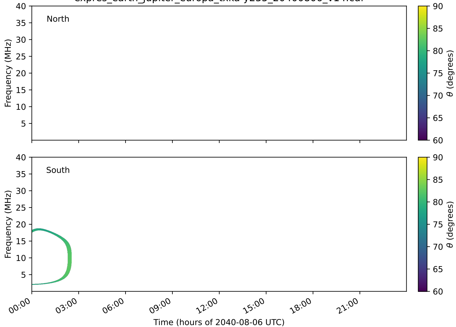
expres_earth_jupiter_europa_txka-y235_20400806_v14.cdf
