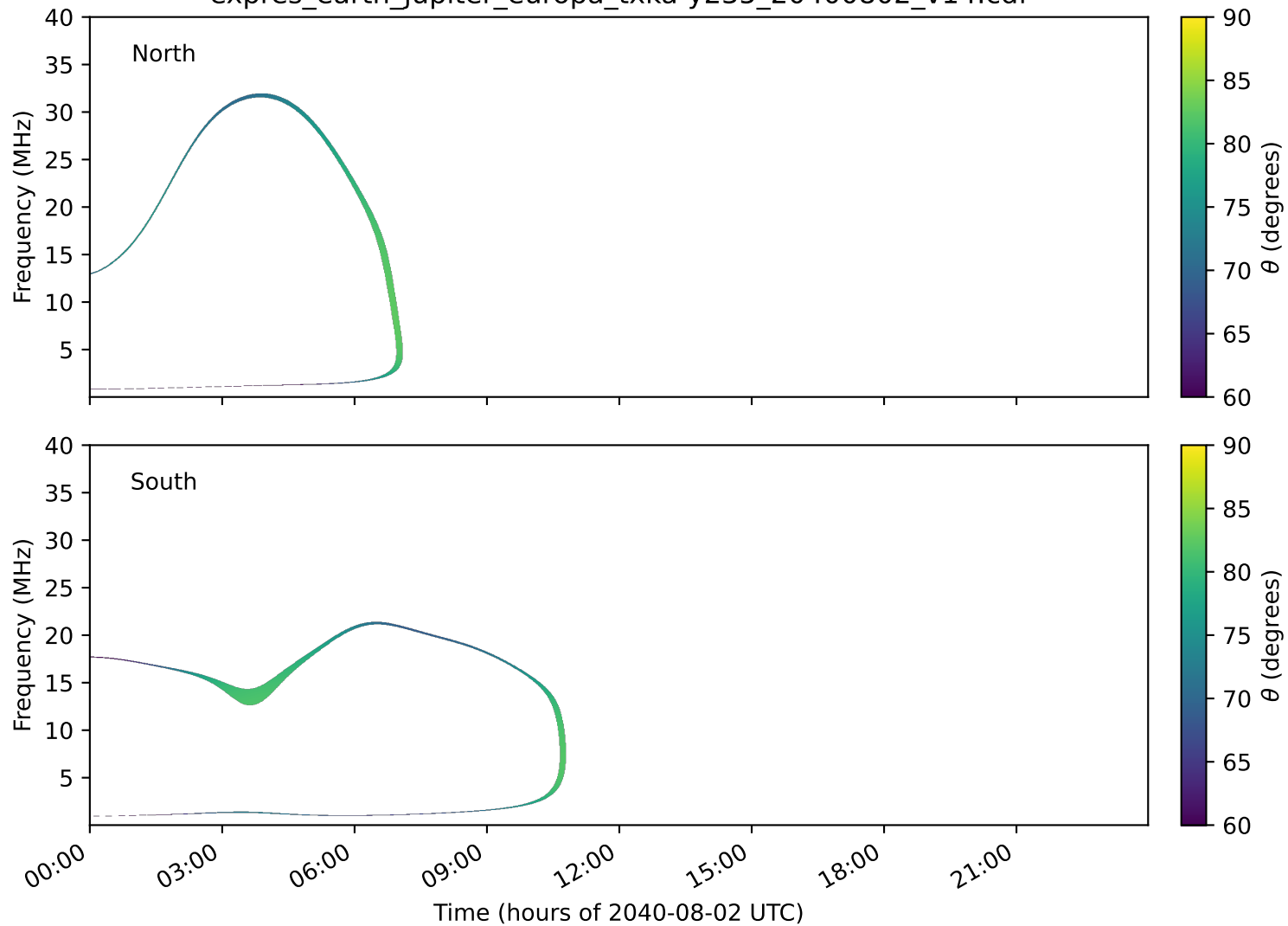
expres_earth_jupiter_europa_txka-y235_20400802_v14.cdf
