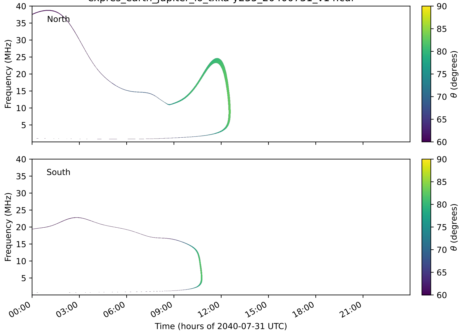
expres_earth_jupiter_io_txka-y235_20400731_v14.cdf
