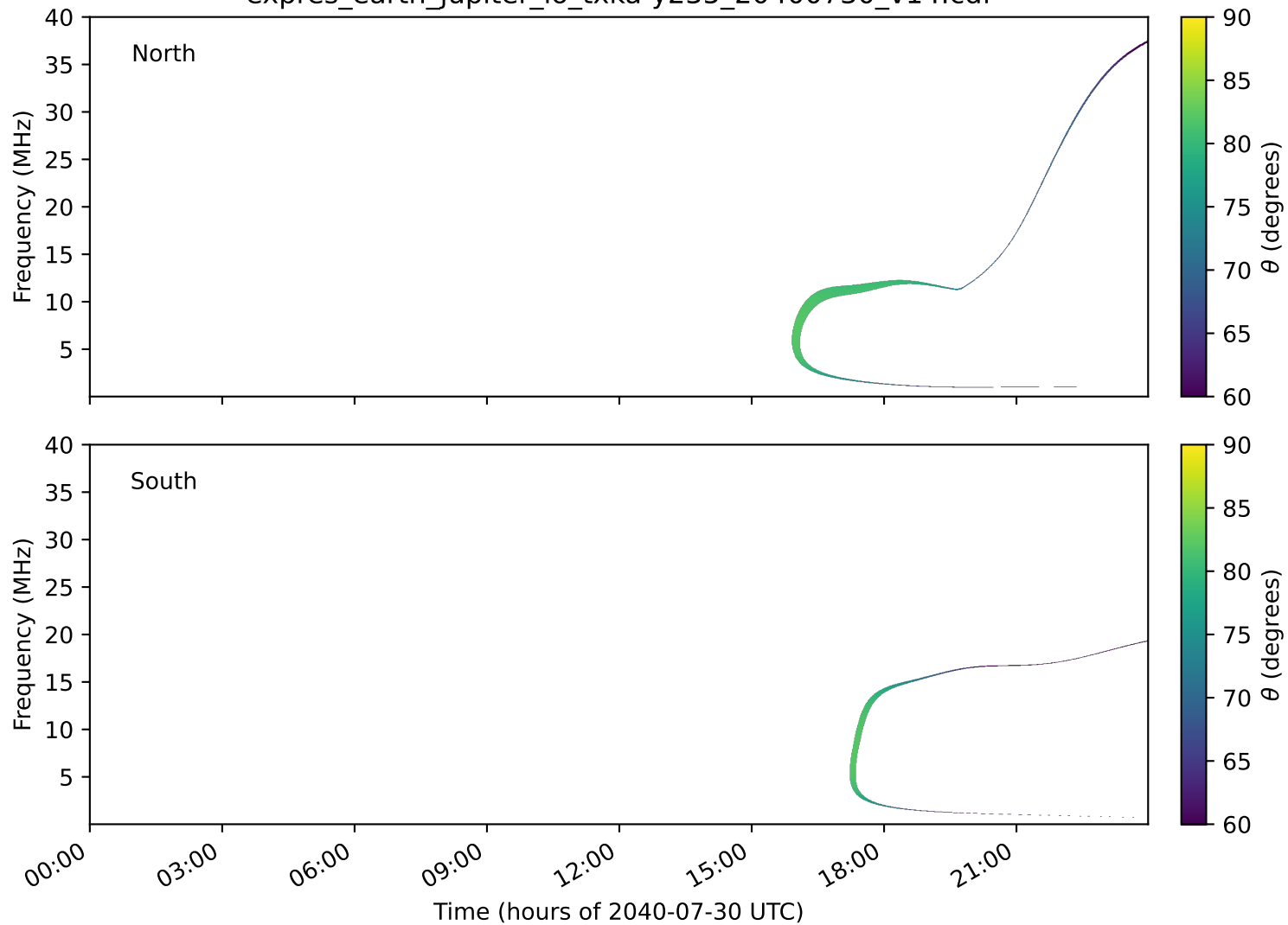
expres_earth_jupiter_io_txka-y235_20400730_v14.cdf
