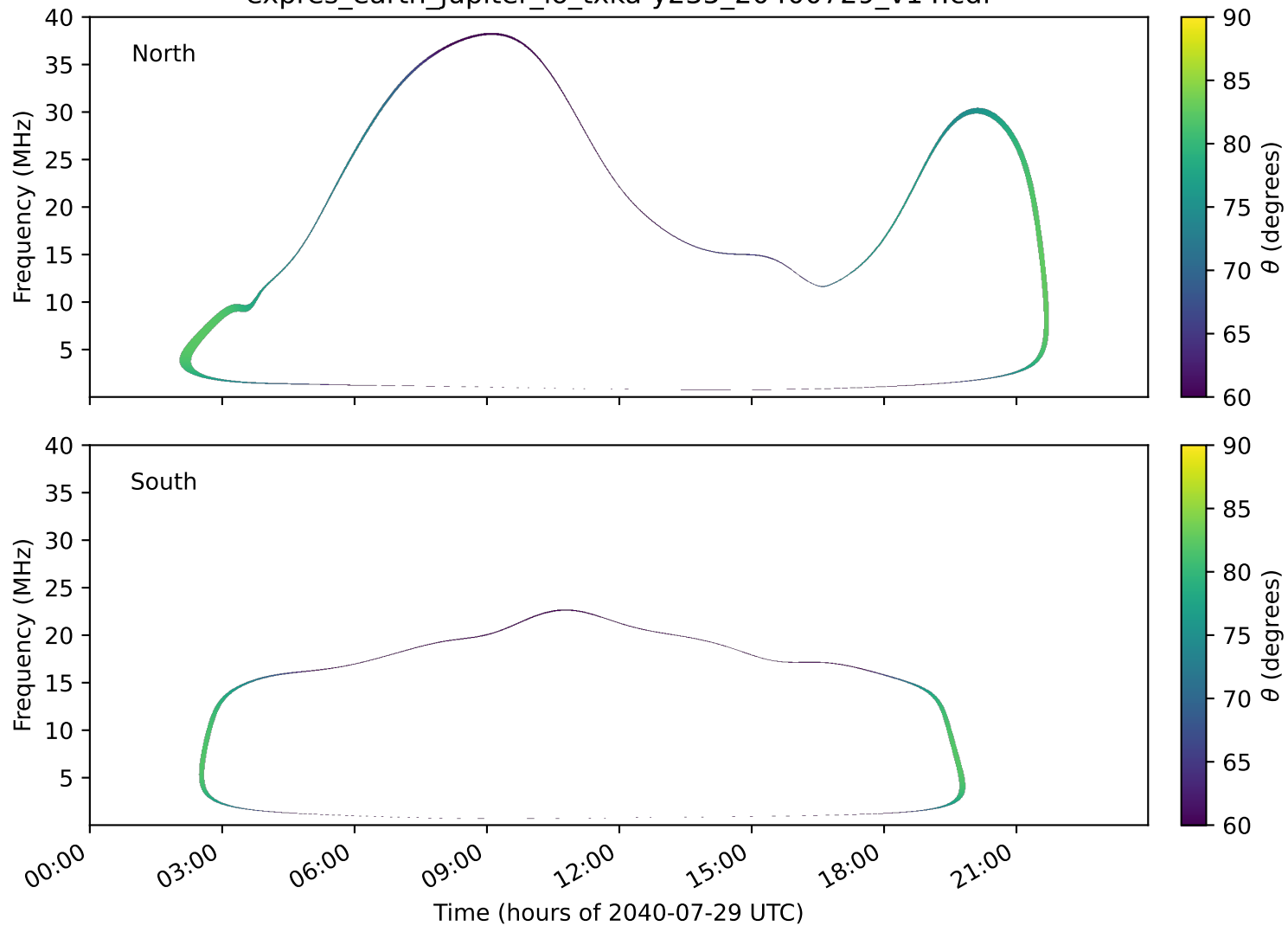
expres_earth_jupiter_io_txka-y235_20400729_v14.cdf
