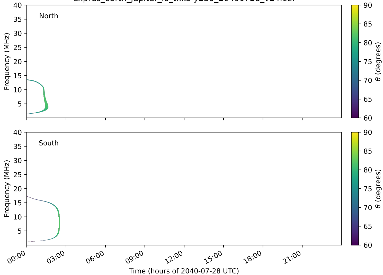
expres_earth_jupiter_io_txka-y235_20400728_v14.cdf
