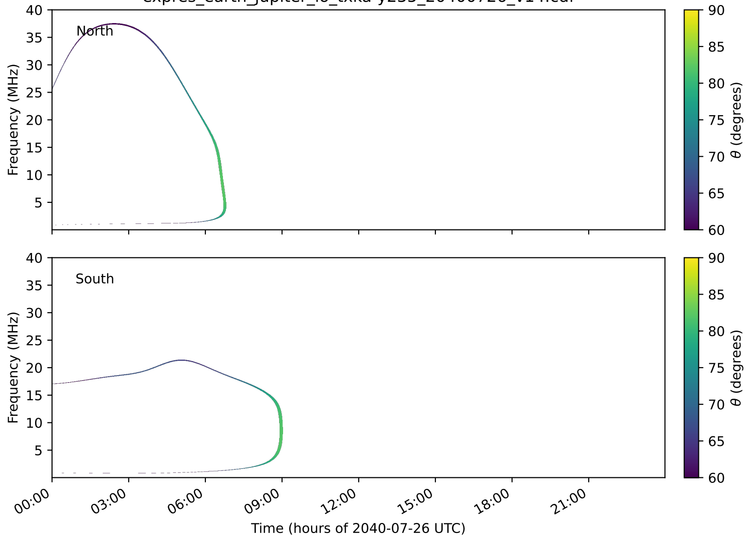
expres_earth_jupiter_io_txka-y235_20400726_v14.cdf
