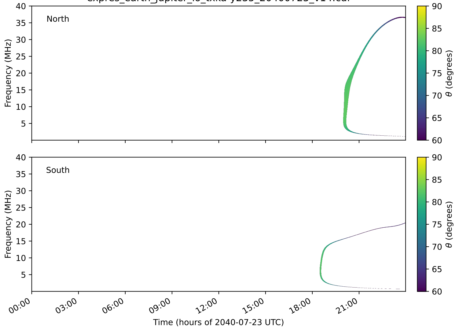
expres_earth_jupiter_io_txka-y235_20400723_v14.cdf
