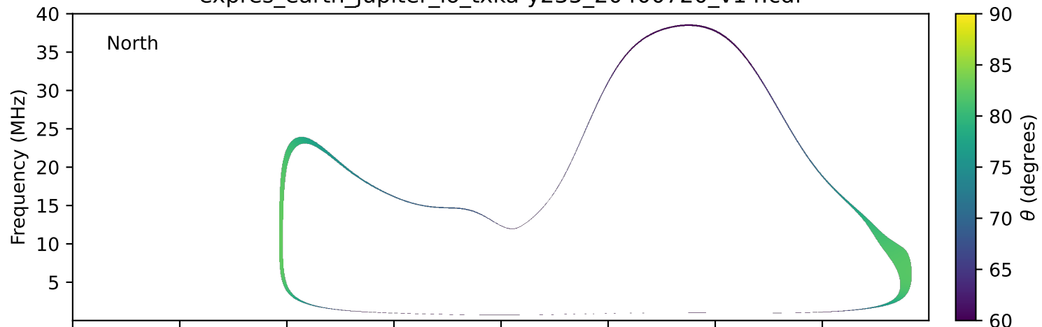
expres_earth_jupiter_io_txka-y235_20400720_v14.cdf
