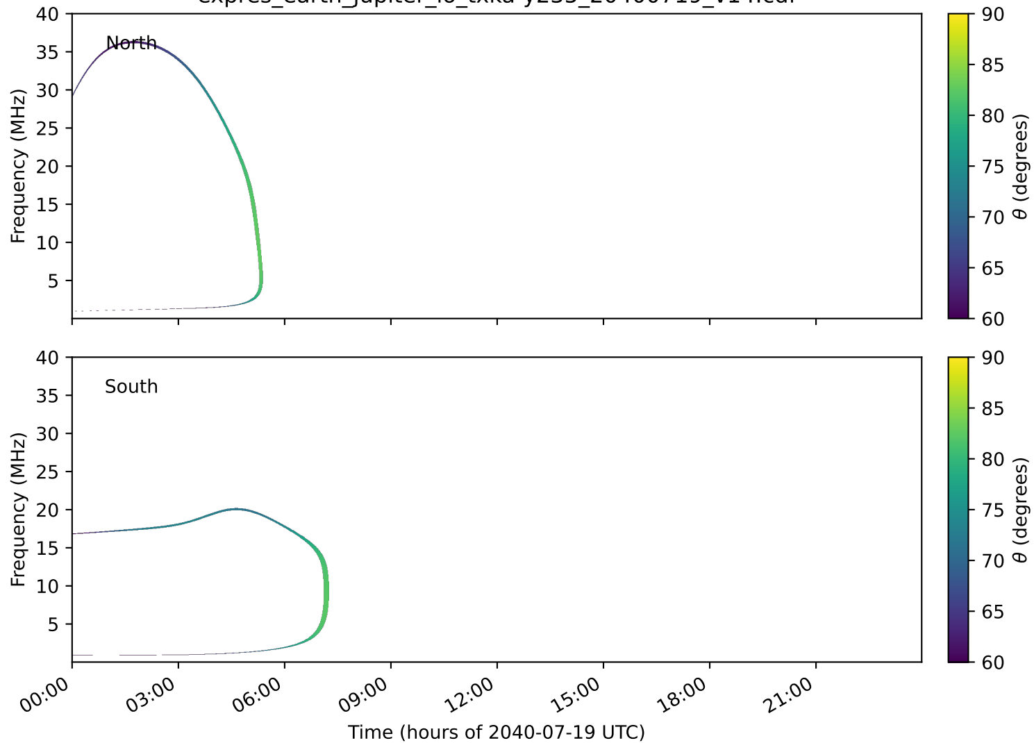
expres_earth_jupiter_io_txka-y235_20400719_v14.cdf
