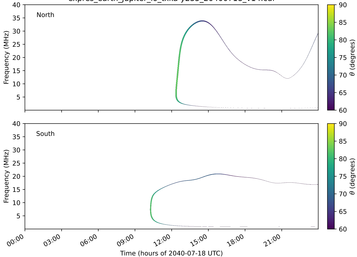
expres_earth_jupiter_io_txka-y235_20400718_v14.cdf
