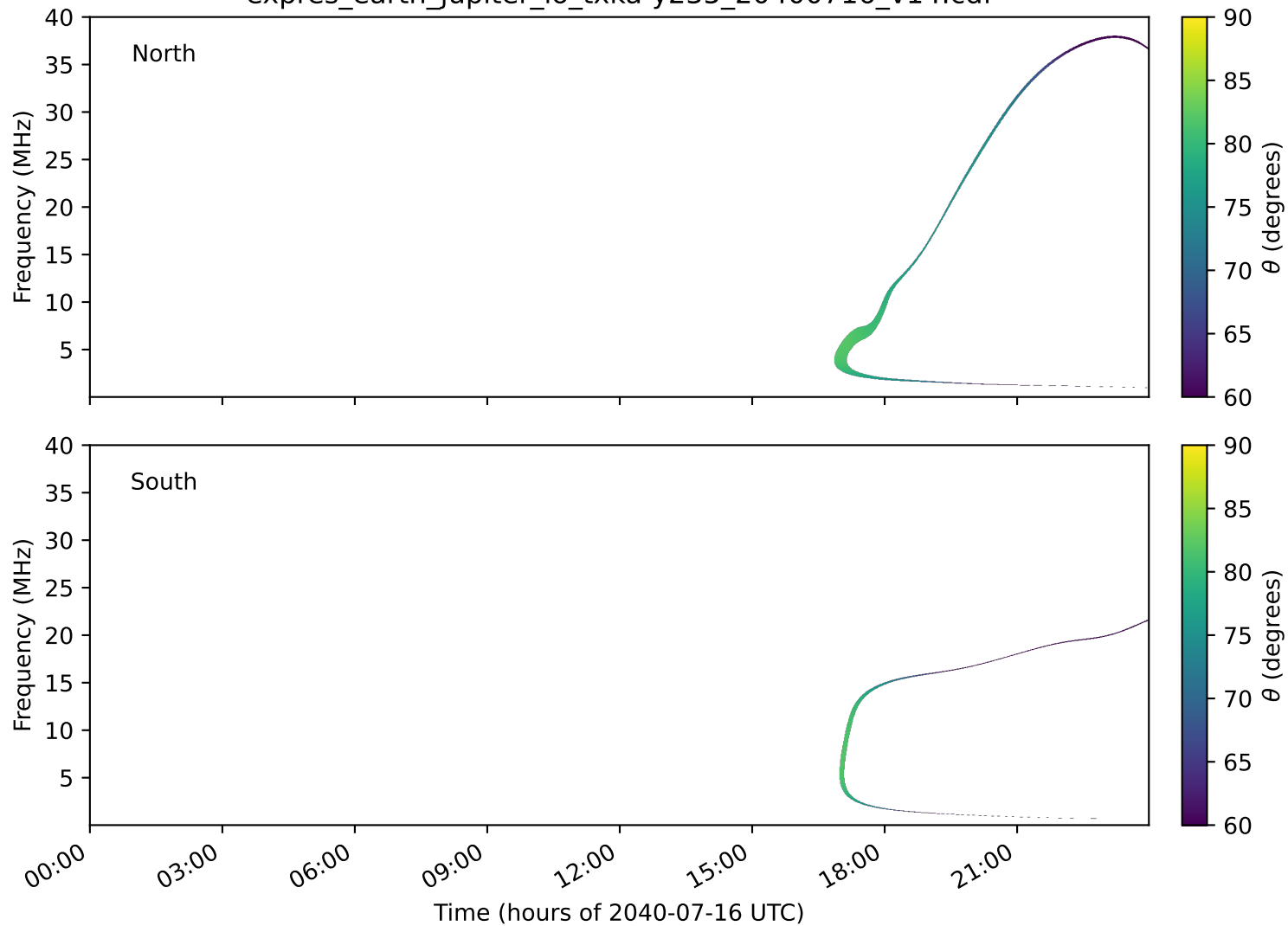
expres_earth_jupiter_io_txka-y235_20400716_v14.cdf
