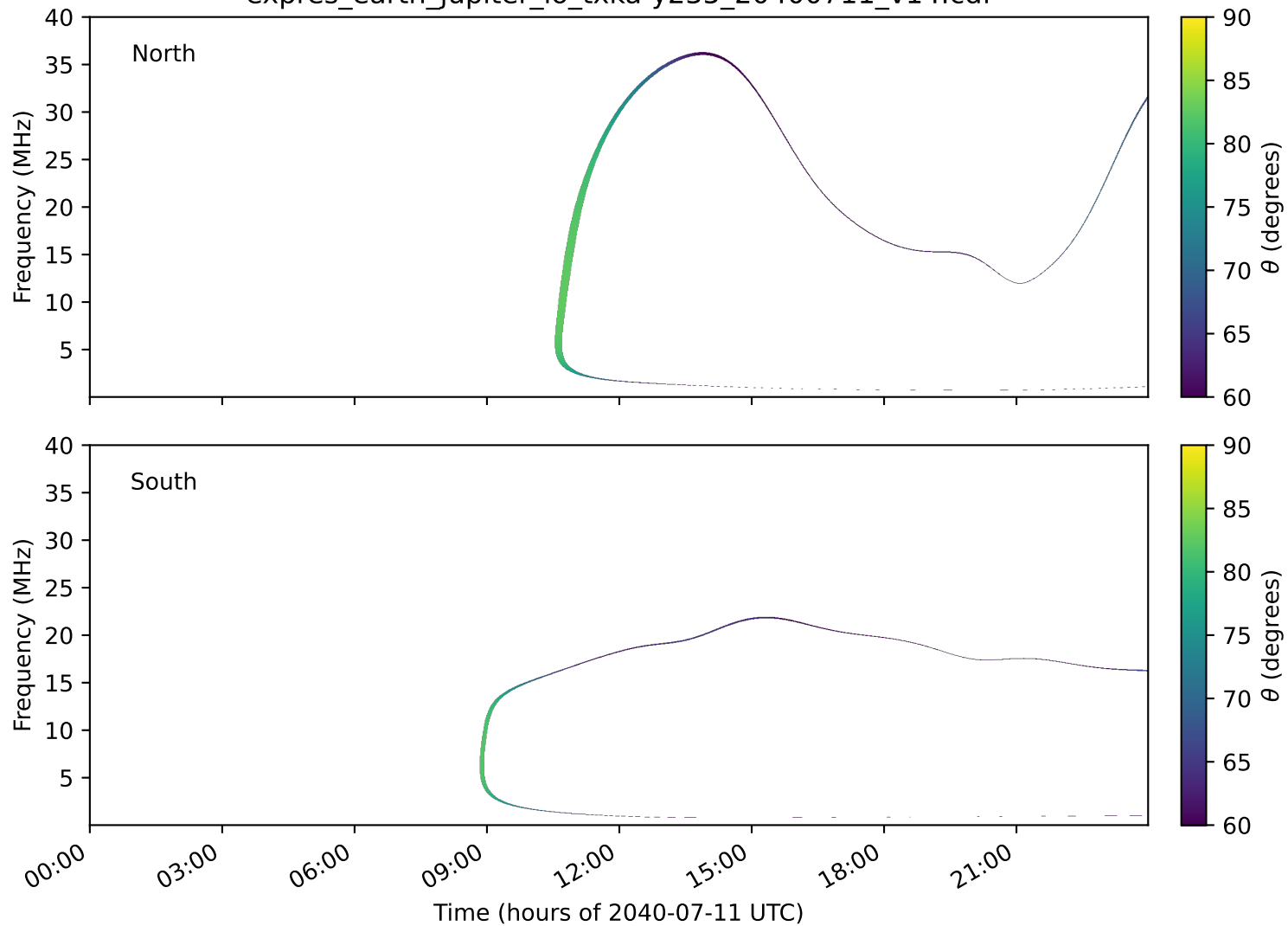
expres_earth_jupiter_io_txka-y235_20400711_v14.cdf
