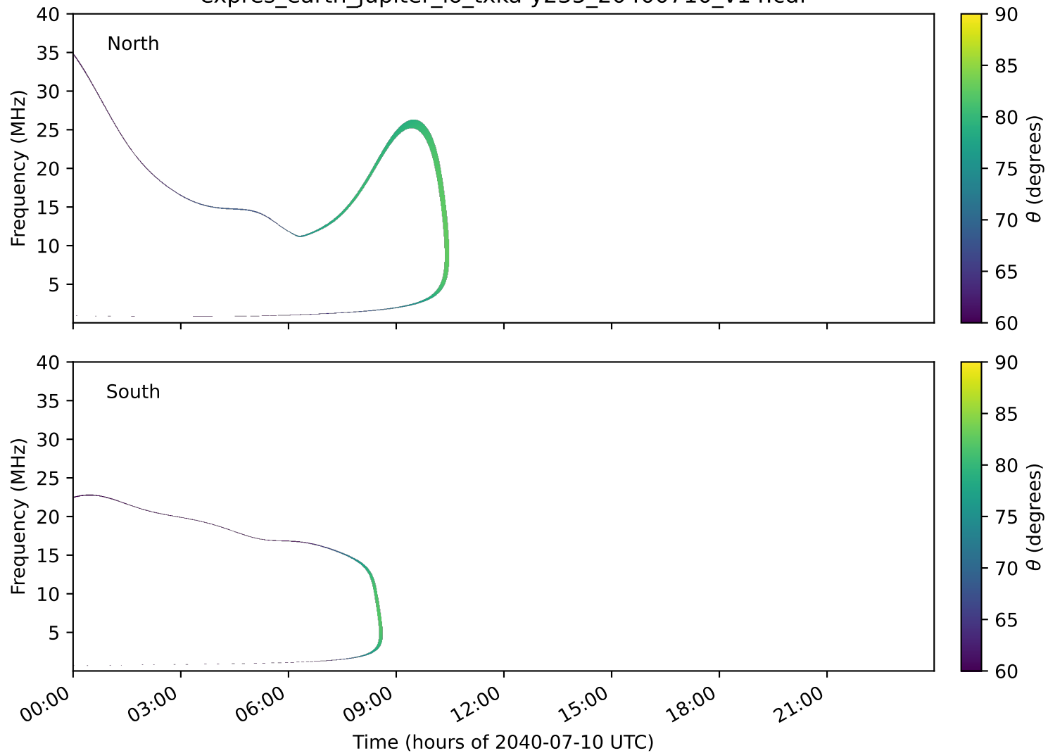
expres_earth_jupiter_io_txka-y235_20400710_v14.cdf
