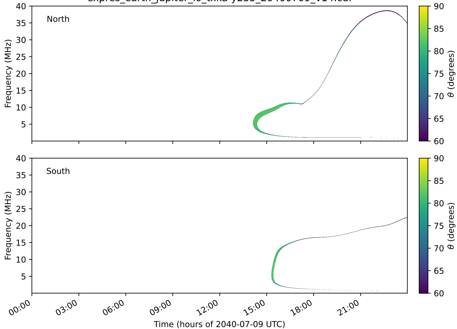
expres_earth_jupiter_io_txka-y235_20400709_v14.cdf
