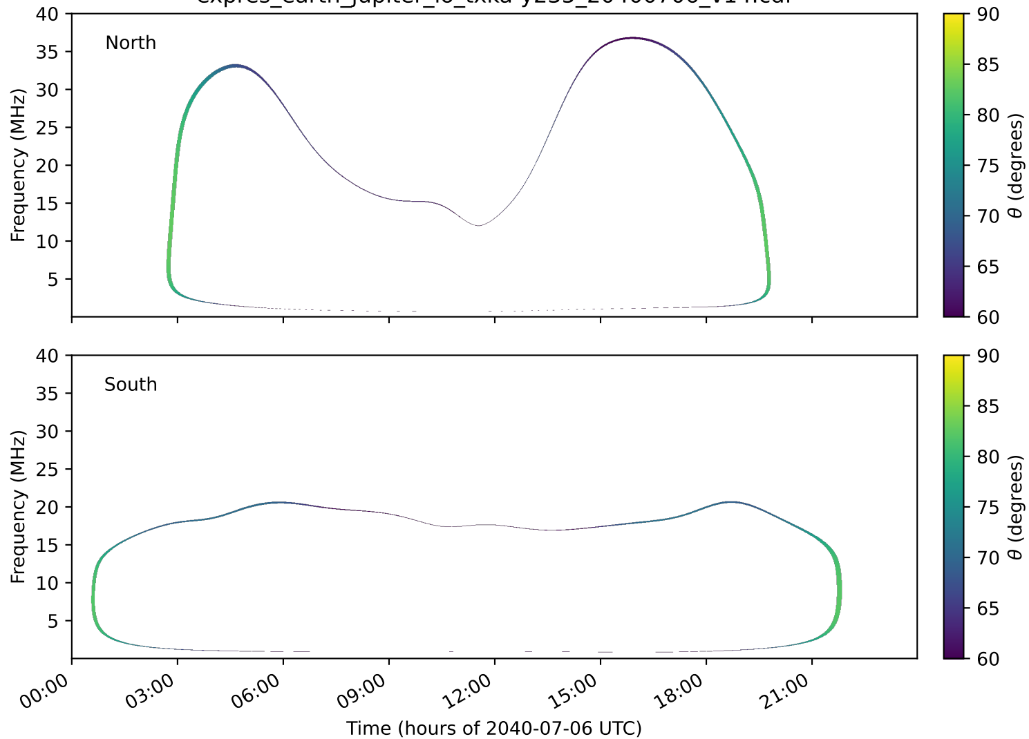
expres_earth_jupiter_io_txka-y235_20400706_v14.cdf
