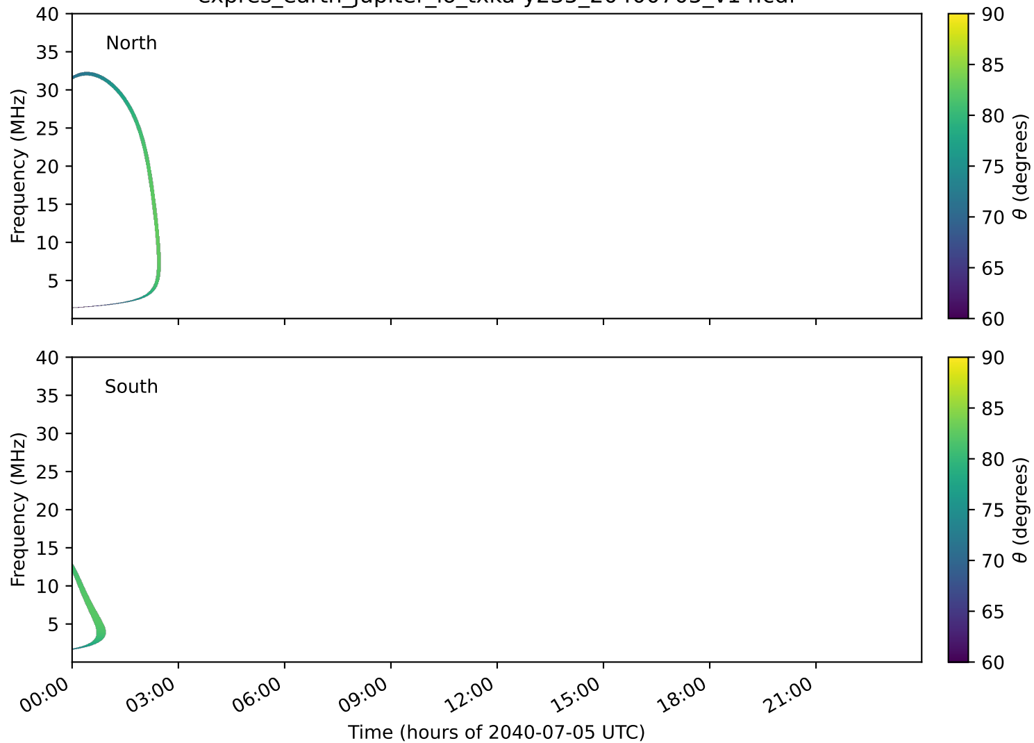
expres_earth_jupiter_io_txka-y235_20400705_v14.cdf
