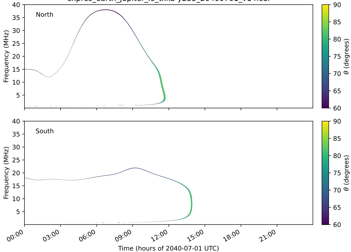
expres_earth_jupiter_io_txka-y235_20400701_v14.cdf
