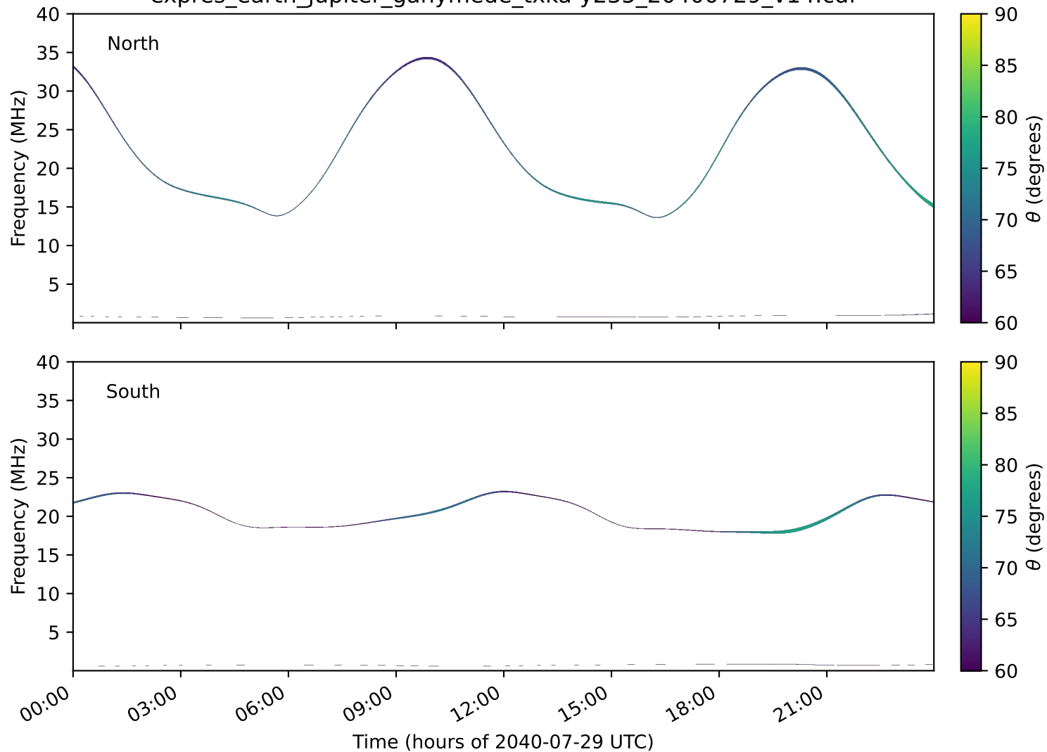
expres_earth_jupiter_ganymede_txka-y235_20400729_v14.cdf
