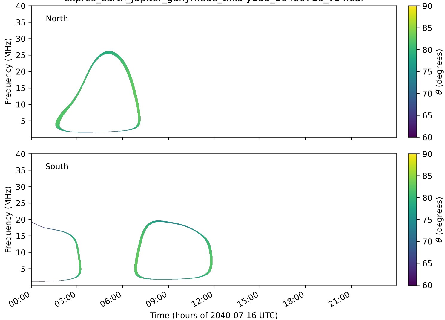
expres_earth_jupiter_ganymede_txka-y235_20400716_v14.cdf
